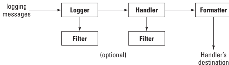
Figure 28-2: Logging architecture
