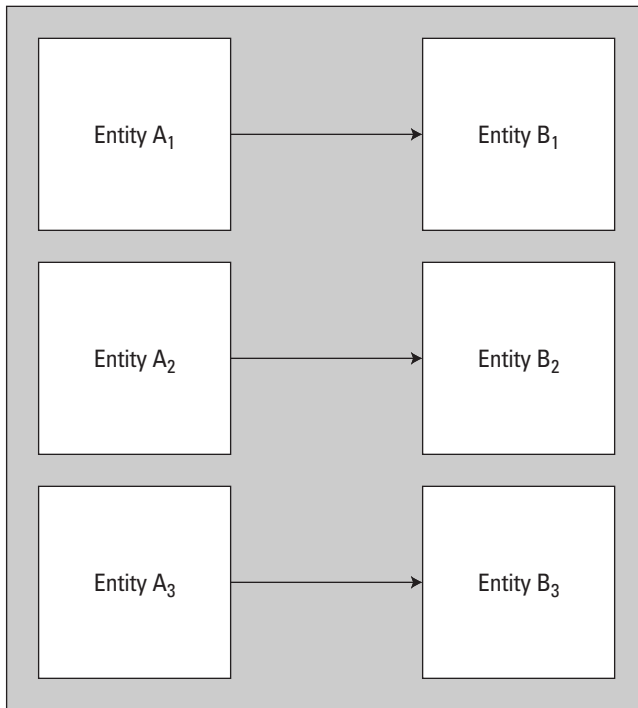
Figure 16-6: One-to-one relationship
