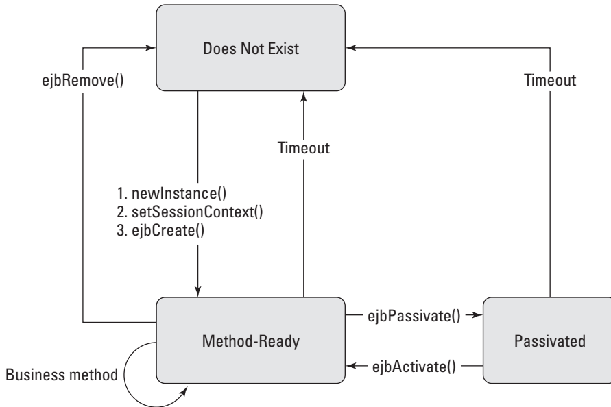
Figure 15-5: Stateful-session-bean lifecycle.
