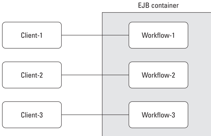
Figure 15-4: Stateful-session-bean model
