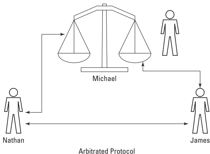
Figure 13-9: Arbitrated protocol
