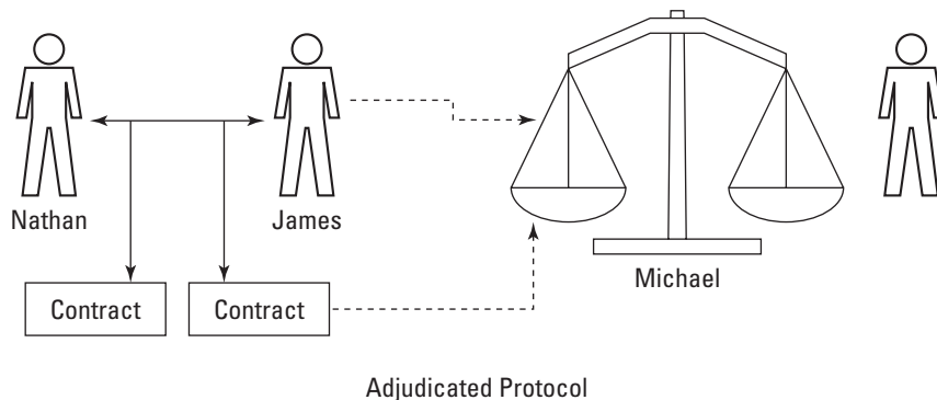
Figure 13-8: Adjudicated protocol
