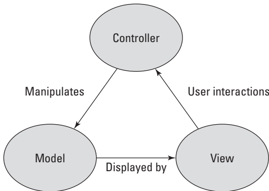
Figure 1-3: MVC pattern
