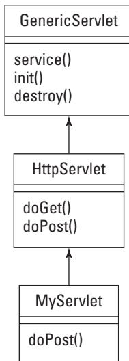
Figure 5-2: The servlet inheritance hierarchy
