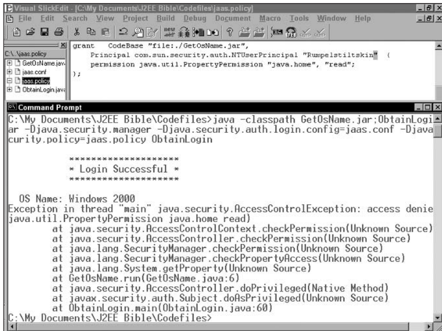
Figure 12-3: An unauthorized user sees error messages bleeding all over the screen.
