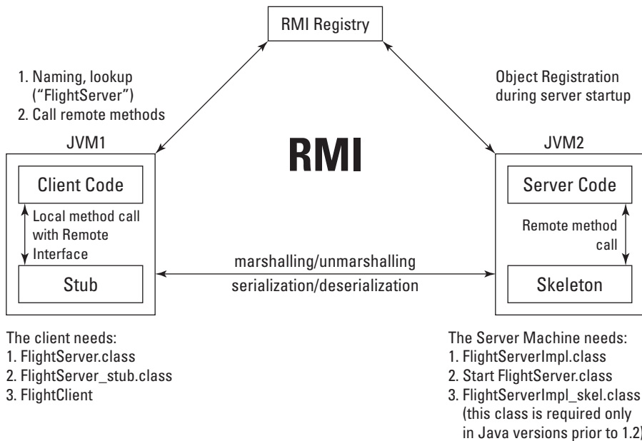
Figure 4-1: The Flight Server example contains these RMI components.
