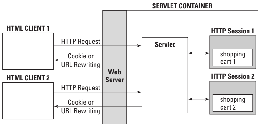
Figure 5-4: Session tracking
