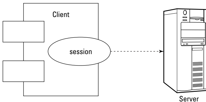
Figure 23-2: Client-maintained session
