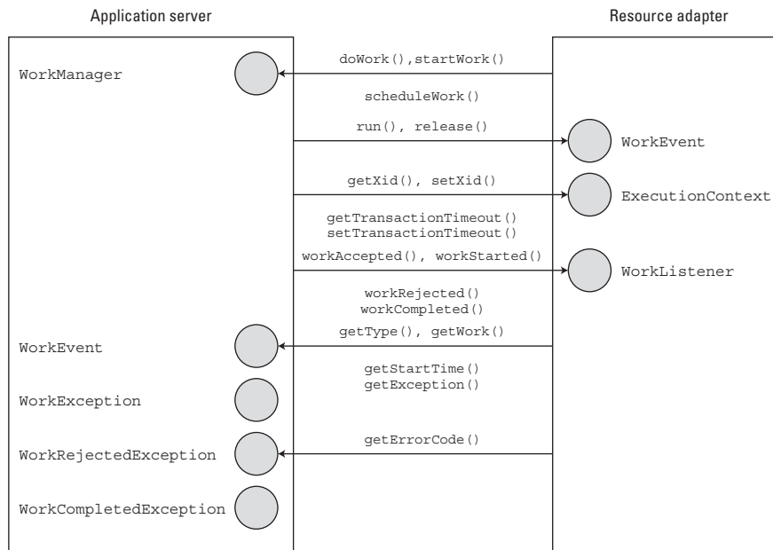
Figure 19-3: Work-management interfaces
