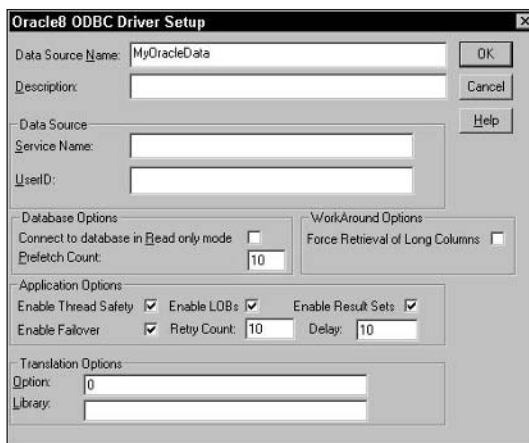
Figure 18-2: How to configure the Oracle ODBC driver
