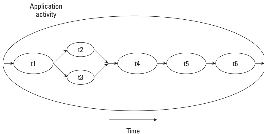
Figure 10-10: This logical long-running transaction does not encounter failure.
