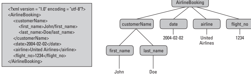
Figure 2-2: A DOM parser's memory structure
