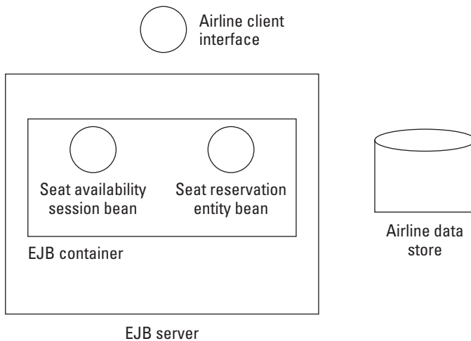
Figure 14-3: Airline reservation example using session and entity beans
