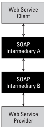
Figure 21-2: Intermediaries are part of the SOAP message exchange model.
